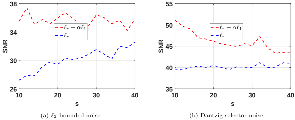
Fig. 4.3. Recovery performance of two algorithms.
