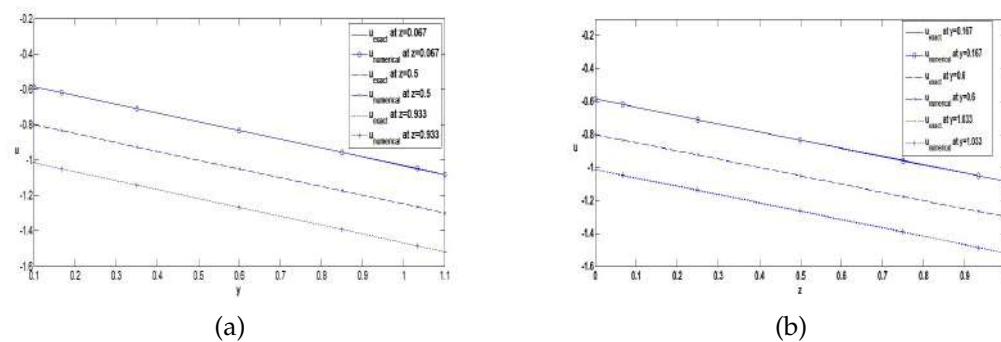
Figure 9: Velocity component ( u ) profile using DSCDQM-RSK with C_1=C_2=C_5=1 , t=1\text{msec} and \gamma=1.13 at different value of y, z .
