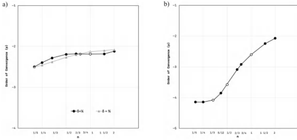
Figure 7: Order of convergence of L2 Error computed over N_y = \{12, 24, 32, 48, 96\} for the Navier non-linear law with \zeta=0.1 or \text{Kn}=0.1 and m=2 (but shared by all slip models), and using \Lambda = \Lambda_{\text{opt}} , as function of the power-law exponent n using the LSOB scheme. Panel (a): Setting \delta_y = 1/4 and \delta_y = 3/4 . Panel (b): Setting \delta_y = 0 . In panel (b), the hollow markers in both panels denote singularities in the continuous line; they correspond to the cases n=1/2 and n=1/3 where the rate of convergence is not defined since numerical and analytical solutions exactly match at \Lambda = \Lambda_{\text{opt}} .
