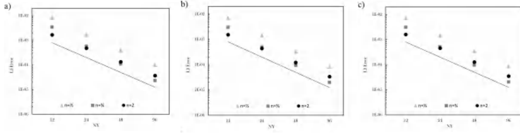
Figure 8: Mesh convergence plots in a 2D diagonal inclined channel using the LSOB scheme, with \delta_{y'} = \delta_y \cos\theta = \frac{1}{4} \frac{\sqrt{2}}{2} wall boundary node distance, fixing \Lambda = 3/16 , for a non-Newtonian power-law fluid with exponents n=1/2 (triangle), n=3/4 (square) and n=2 (circle), where continuous straight line indicates a slope -2. Panel (a): No-slip BC ( \zeta=0 or \text{Kn}=0 ). Panel (b): Navier linear slip BC ( \zeta=0.1 or \text{Kn}=0.1 ). Panel (c): Navier non-linear slip BC ( \zeta=0.1 or \text{Kn}=0.1 and m=2 ).
