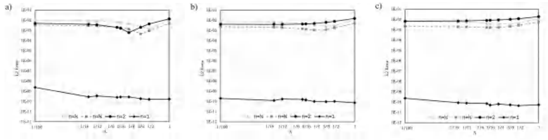
Figure 12: Effect of TRT relaxation parameter \Delta in a 3D pipe on the numerical error with LSOB scheme, on a coarse mesh ( R=N_y=N_z=12 ), for a Newtonian fluid n=1 (diamond) and non-Newtonian power-law fluid with exponents n=1/2 (triangle), n=3/4 (square) and n=2 (circle). Panel (a): No-slip BC ( \zeta=0 or \text{Kn}=0 ). Panel (b): Navier linear slip BC ( \zeta=0.1 or \text{Kn}=0.1 ). Panel (c): Navier non-linear slip BC ( \zeta=0.1 or \text{Kn}=0.1 and m=2 ).
