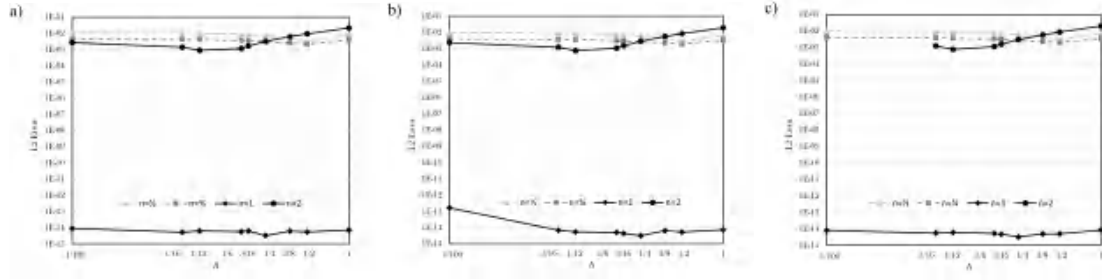
Figure 9: Effect of TRT relaxation parameter \Delta in a 2D diagonal inclined channel on the numerical error with LSOB scheme, on a coarse mesh ( N_y=12 ), for a Newtonian fluid n=1 (diamond) and non-Newtonian power-law fluid with exponents n=1/2 (triangle), n=3/4 (square) and n=2 (circle). Panel (a): No-slip BC ( \zeta=0 or \text{Kn}=0 ). Panel (b): Navier linear slip BC ( \zeta=0.1 or \text{Kn}=0.1 ). Panel (c): Navier non-linear slip BC ( \zeta=0.1 or \text{Kn}=0.1 and m=2 ). All cases consider the generic value \delta_{y'} = \delta_y \cos \theta = \frac{1}{4} \frac{\sqrt{2}}{2} for the wall boundary node distance.
