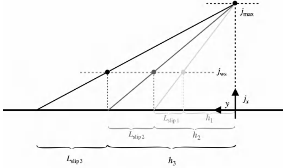
Figure 3: Self similar solutions illustrated across three cases. An increase in the domain resolution (here represented by h ) should not result in a change in slip velocity, for a fixed dimensionless slip length (liquids) or the Knudsen number (gases). The slip length ( L_{\text{slip}} ) scales with h to accommodate self-similarity.
