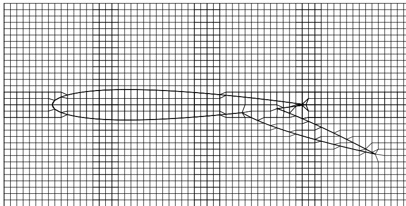
Figure 7: Result of the primary mesh adjustment.
