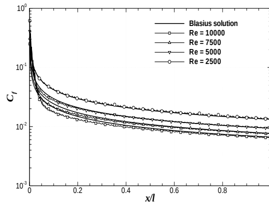
Figure 16: Estimation of the skin-friction coefficient for a non-axis aligned flat plate at M=0.2 for Reynolds numbers of 2,500, 5,000, 7,500, and 10,000 on the mesh shown in Fig. 14.
