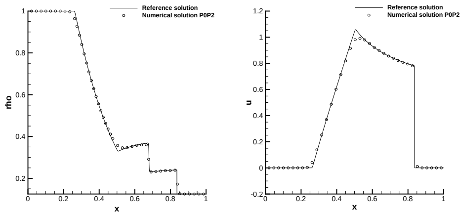
Figure 4: Profiles along the positive x -axis of density (left) and velocity (right) at time t=0.2 .
