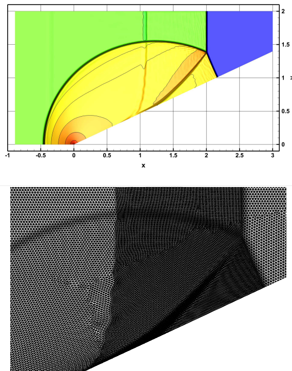
Figure 11: Top: 21 equidistant density contours from \rho = 1.2 to \rho = 3 for the single Mach reflection problem ( M_s = 1.7, \alpha = 25^\circ ). Bottom: zoom into the mesh at the final time t = 1.2 .
