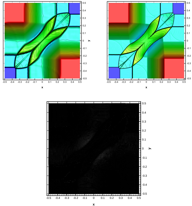
Figure 12: Top left: 50 equidistant density contour lines from \rho=0.14 to \rho=0.98 for the numerical solution obtained with our third order unstructured Lagrangian one-step WENO finite volume scheme for the two-dimensional Riemann problem RP1 at t=0.2 . Top right: Same contour lines for the reference solution. Bottom: computational mesh of the Lagrangian scheme at the final time t=0.2 .
