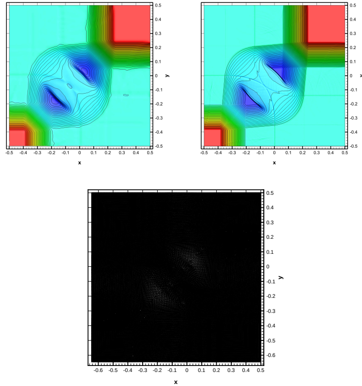
Figure 13: Top left: 51 equidistant density contour lines from \rho=0.27 to \rho=0.98 for the numerical solution obtained with our third order unstructured Lagrangian one-step WENO finite volume scheme for the two-dimensional Riemann problem RP2 at t=0.2 . Top right: Same contour lines for the reference solution. Bottom: computational mesh of the Lagrangian scheme at the final time t=0.2 .
