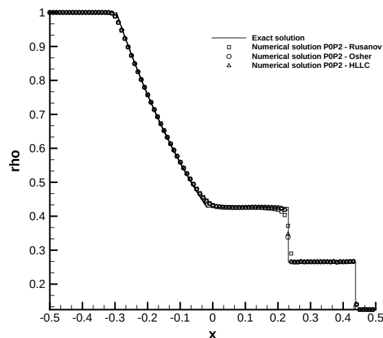
Figure 3: Sod shock tube test. Third order accurate numerical results obtained using three different numerical fluxes (Rusanov, Osher and HLLC) and comparison with the exact solution (solid line) at time t=0.25 .
