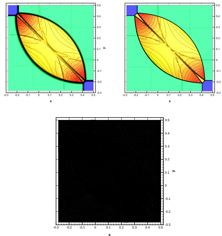
Figure 14: Top left: 51 equidistant density contour lines from \rho=0.53 to \rho=1.9 for the numerical solution obtained with a third order unstructured Lagrangian one-step WENO finite volume scheme for the two-dimensional Riemann problem RP3 at t=0.245 . Top right: Same contour lines for the reference solution. Bottom: computational mesh of the Lagrangian scheme at the final time t=0.245 .
